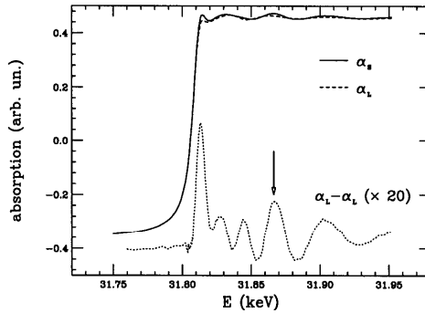
Figure 1: K-edge of solid ( \alpha_S , solid curve) and liquid ( \alpha_L , dashed curve) Te in graphite at 400°C and 470°C respectively. The chosen energy point for temperature scan is indicated by the vertical arrow on the difference curve.
