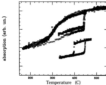
Figure 2: Single energy X-ray absorption scan vs. temperature for Te particles confined in NaCl (upper curve) and graphite (lower curve).
