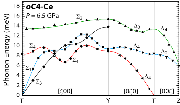
Figure 2: Measured phonon dispersion relations for Ce- oC4 at 6.5 GPa. The symbols distinguish \mathbf{q} -scans with different momentum offsets relative to the center of the Brillouin zone: \blacktriangle (151)–(051)–(041)–(04½); \bullet (201)–(301); \blacksquare (200)–(300); \blacklozenge (061)–( \bar{1} 61); \blacktriangleright (210)–(220); \blacktriangleleft (210)–(200); \blacktriangledown (201)–(20½). The experimental uncertainties of the phonon energies correspond approximately to the symbol size. The lines are guides to the eye, and the branches are labeled as in [2].
