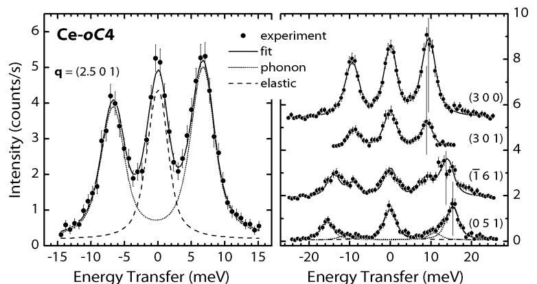
Figure 1: Selected IXS spectra of Ce- oC4 at 6.5 GPa for different momentum transfers \mathbf{q} . When \mathbf{q} is reduced to the first Brillouin zone, (2.5 0 1) corresponds to (\frac{1}{2} 0 0) , i.e. halfway along the \Gamma -Y line. The spectra in the right panel are collected with momentum transfers all corresponding to the Y point, (100), but with emphasis on different phonon branches. The spectra are offset vertically for clarity.
