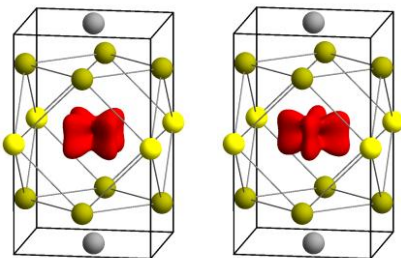
Fig. 1 Crystal structure of CeCoIn 5 and the two possible orientations of the cerium \Gamma_7 crystal-field ground state. Both 4f orbitals have the same |+5/2\rangle admixture |\alpha| but different signs of \alpha .
