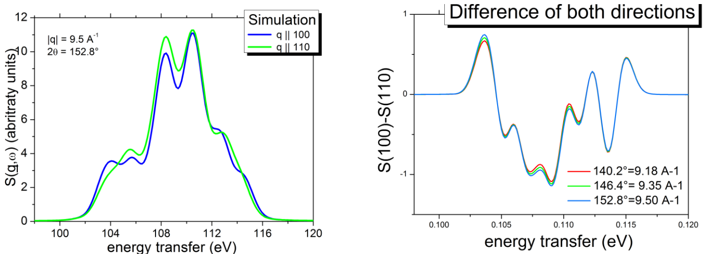
Fig. 3: Simulation of the scattering function S(\mathbf{q},\omega) for \mathbf{q} \parallel \langle 100 \rangle and \mathbf{q} \parallel \langle 110 \rangle and |\mathbf{q}| = 9.5 \text{ \AA}^{-1} which corresponds to the highest scattering angle.
