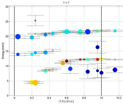
Figure 1: sample time-of-flight neutron data showing the magnetic and phonon contributions to S(Q, E)
