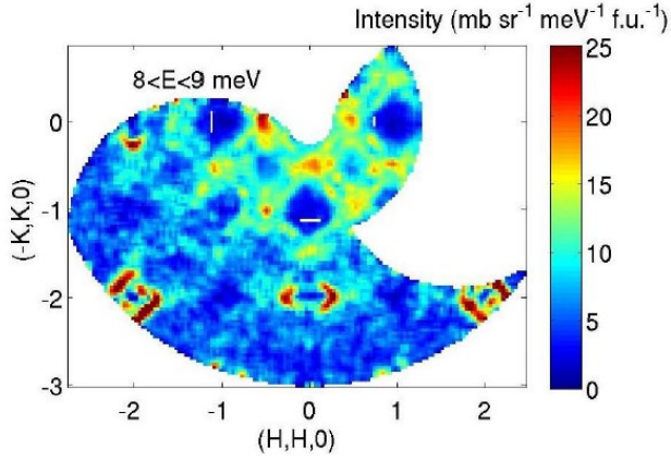
Figure 1: sample time-of-flight neutron data showing the magnetic and phonon contributions to S(Q, E)
